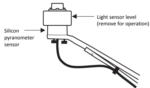
Leveling the Sensor on the Light Sensor Bracket
